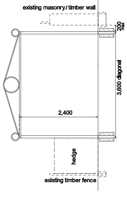
TPK24 - Elevation 1:50
