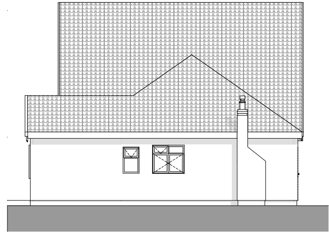
E4 | Right Elevation (Existing) 1:50
